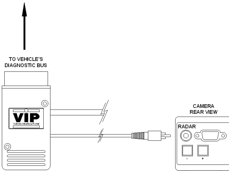
Figure 2.5.3 VIP connection to Video Camera
